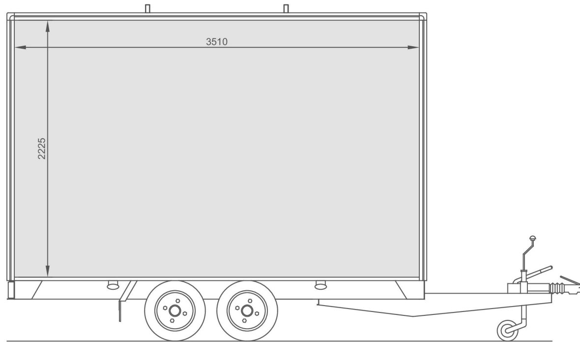
OFFSIDE VIEW (CLOSED)
